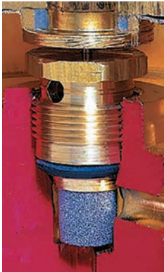
One piece encapsulated seat with internal filter
