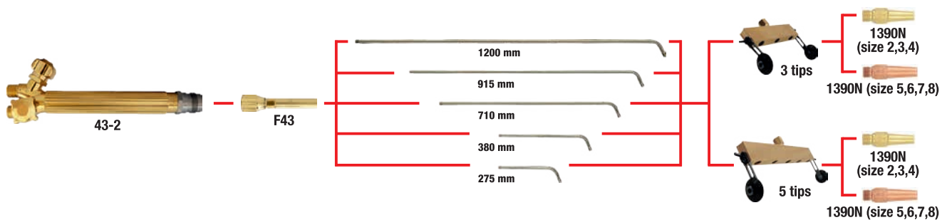
ALTERNATIVE FUEL TIPS PERFORMANCE DATA CHART
